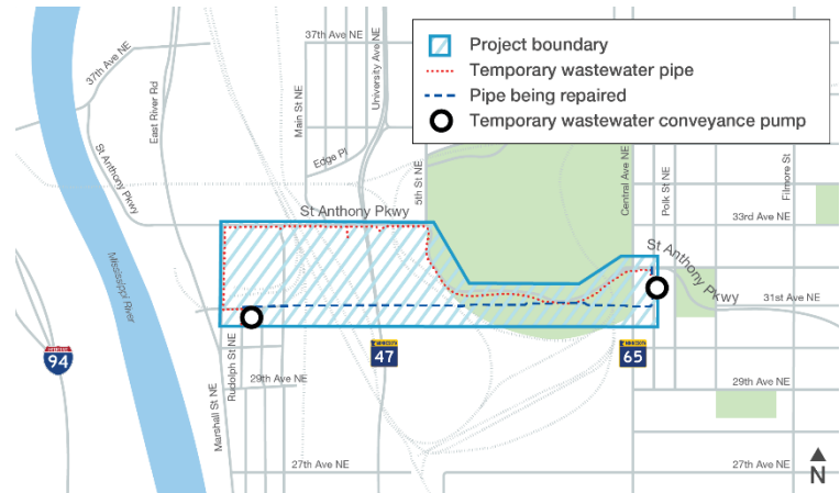
Image caption: project boundary for the sewer pipe rehabilitation in northeast Minneapolis showing the route for the temporary wastewater conveyance and the pipe being repaired.
