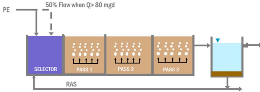
Figure D-2. Alternative 0 – Current Operations Flow Schematic
