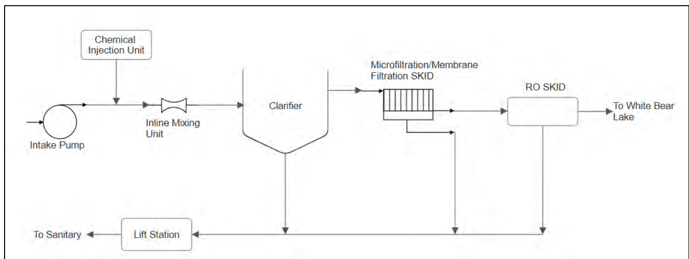
Figure 1 Proposed Lake Augmentation Treatment Process
